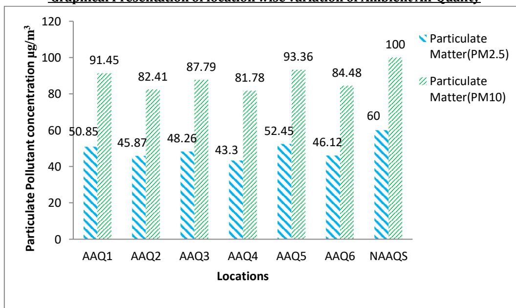
Graphical Presentation of location wise variation of Ambient Air Quality
