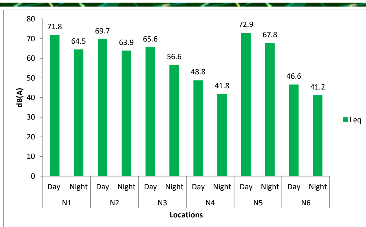
Figure 3.3 Graphical Presentation of Ambient Noise Level
